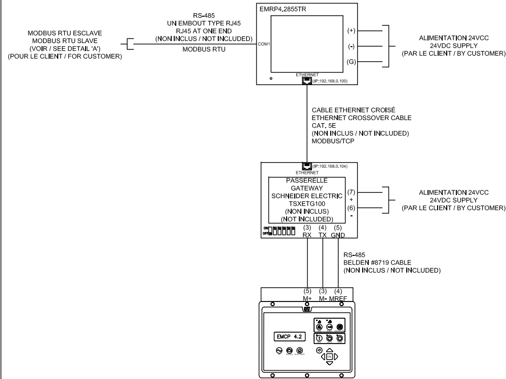
EMRP4.2855TR CONFIGURATION DE BASE BASIC SETUP
