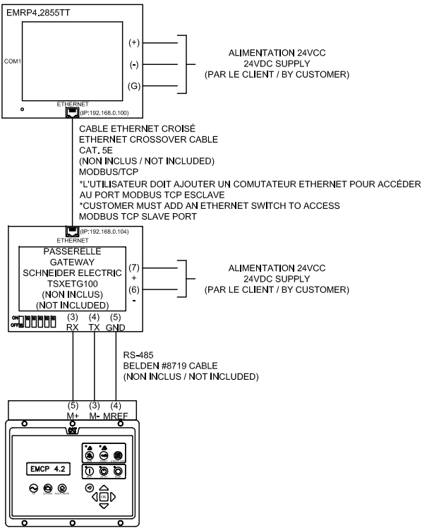
EMRP4.2855TT CONFIGURATION DE BASE BASIC SETUP
